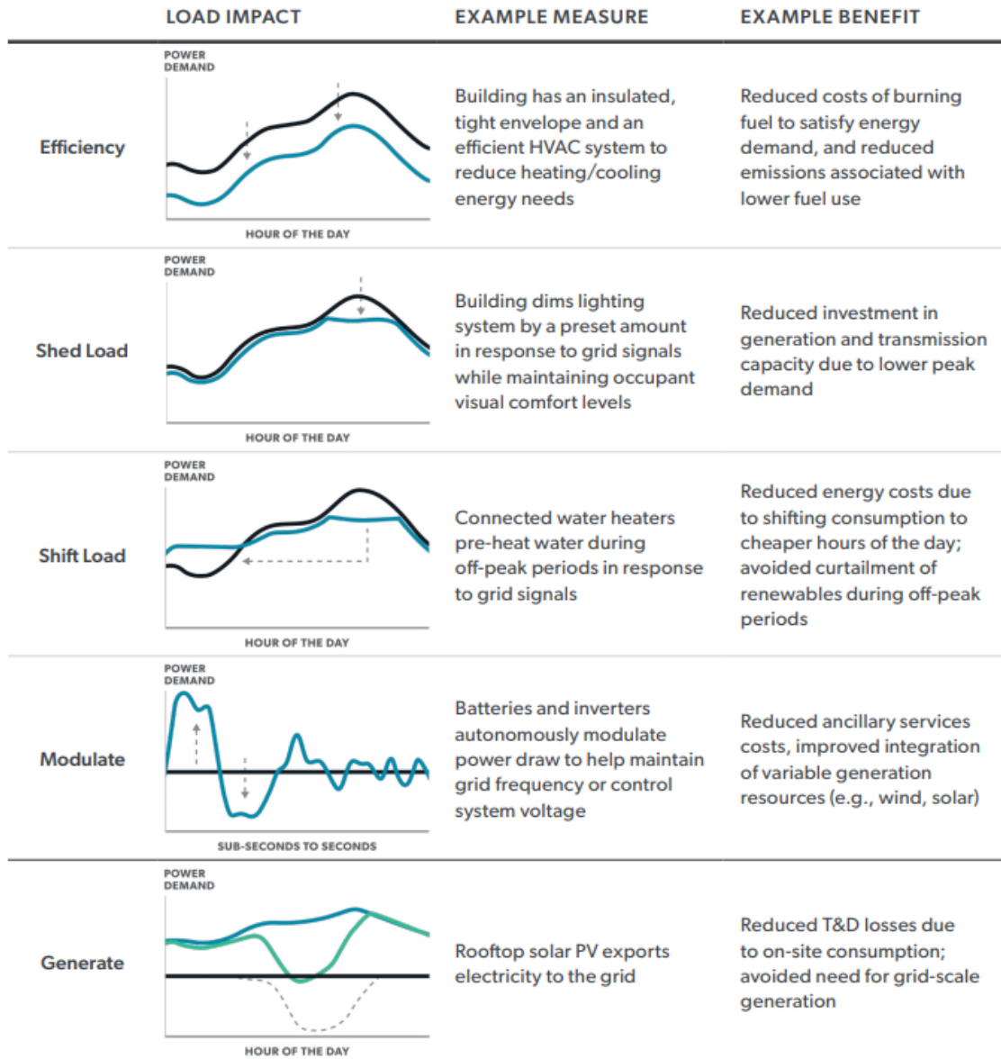
Figure 4. Grid Services that GEBs Can Provide (Source: 2021 DOE GEB Roadmap 1 )
