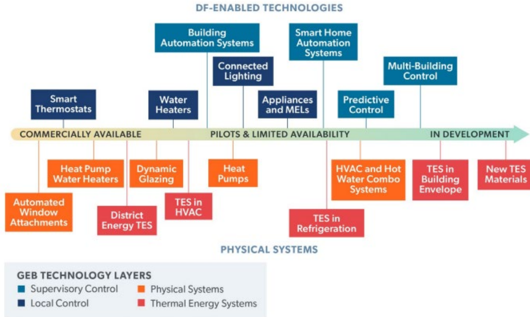
Figure 9. Technology Pipeline Examples for Each GEB Layer (Source: DOE 2021 GEB Roadmap) 66
